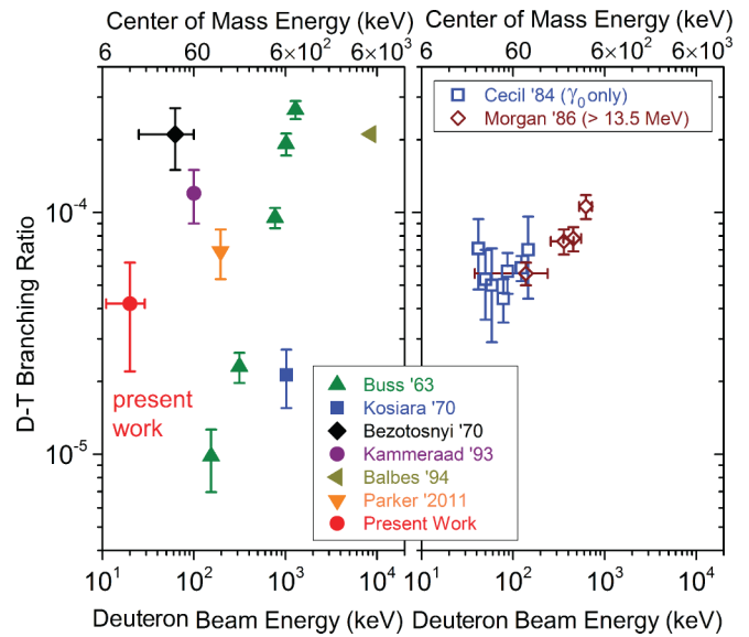
FIG. 4. (Color) D-T branching ratio determined from this ICF implosion work (red solid circle) as compared to earlier work. Branching ratios shown in the left-hand panel include \gamma_0 and \gamma_1 emissions, while only \gamma_0 is considered in the right-hand panel.
